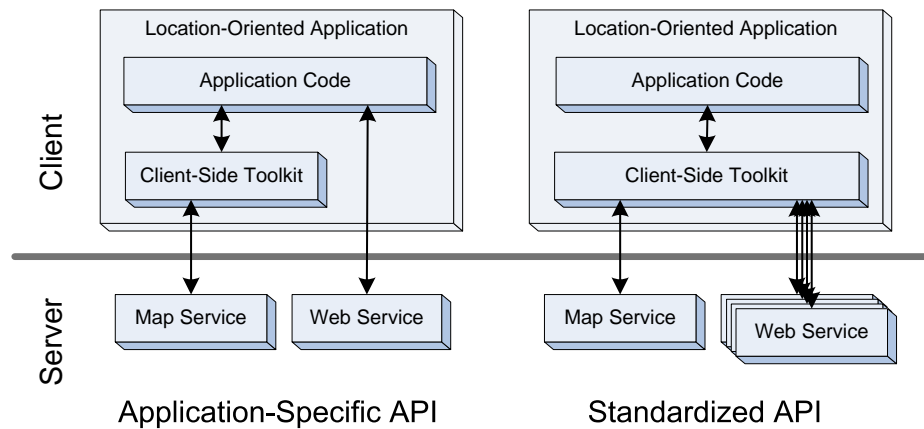
Fig. 2. Architectural comparison between a conventional location-aware service built upon tightly-coupled, application-specific APIs, and a service built upon tiled feeds.
