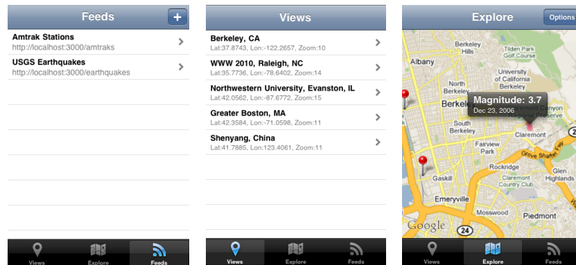
Fig. 4. A basic tiled feed reader. In (a), the user is consuming two location-based services as tiled feeds — locations of nearby Amtrak train stations, and recent M3+ earthquakes from the USGS, respectively. In (b), the user has subscribed to five locations of interest, including Berkeley, CA. In (c), the user selected the Berkeley location, is shown a mashup of Amtrak services and earthquakes at the location of Berkeley, CA.
