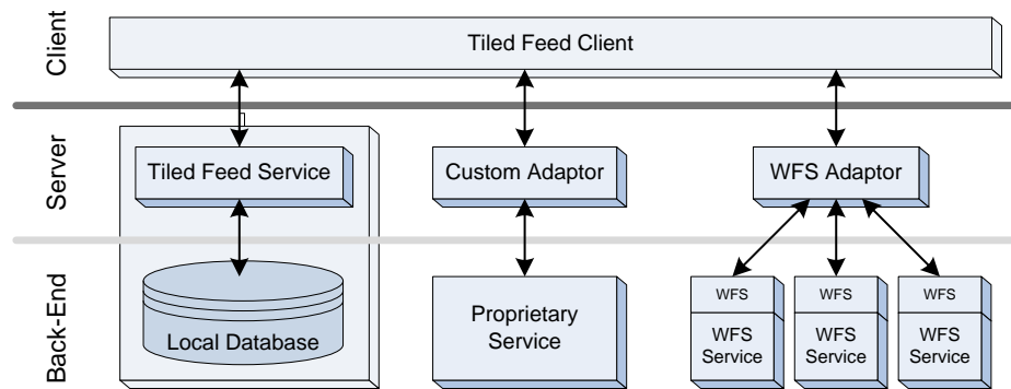
Fig. 3. Implementations of Tiled Feeds atop various geospatial data sources.
