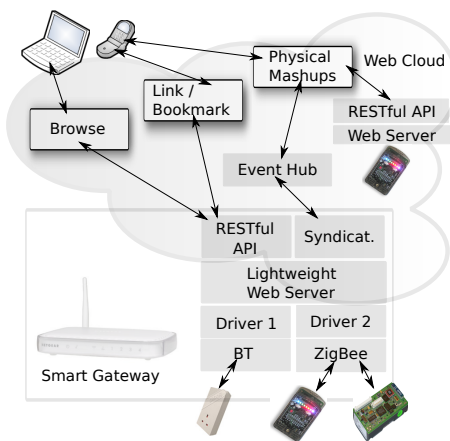
Fig. 1. Web and Internet integration with Smart Gateways (bottom), direct integration (upper-right).
